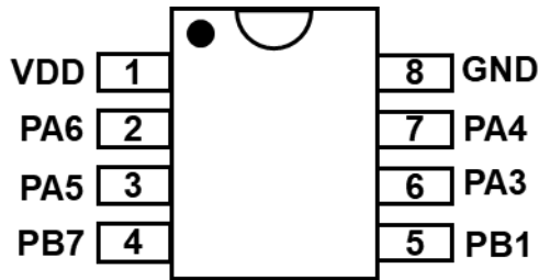
PMS120B-S08A: SOP8 (150mil)
