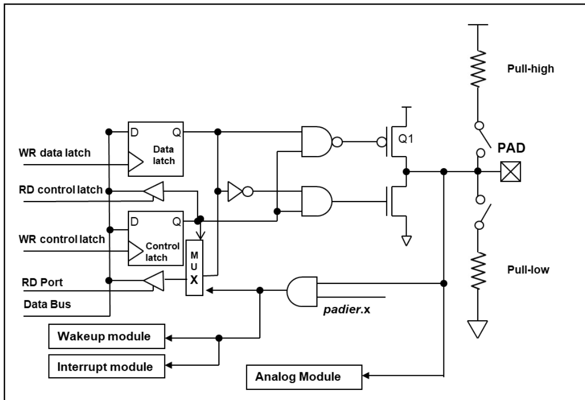
Fig. 18: Hardware diagram of IO buffer
